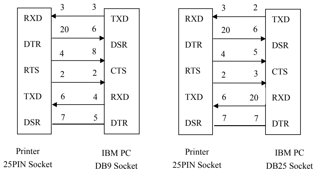
Fig.2-4 Connection between POS90BT and IBM PC Serial Interface Sketch Map
